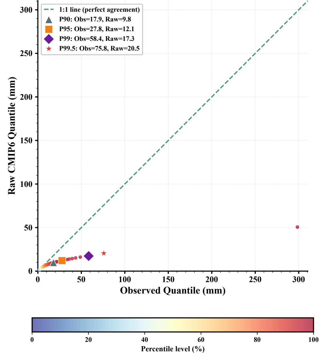
(a) Observed vs Raw CMIP6 QQ-RMSE = 18.98 mm
