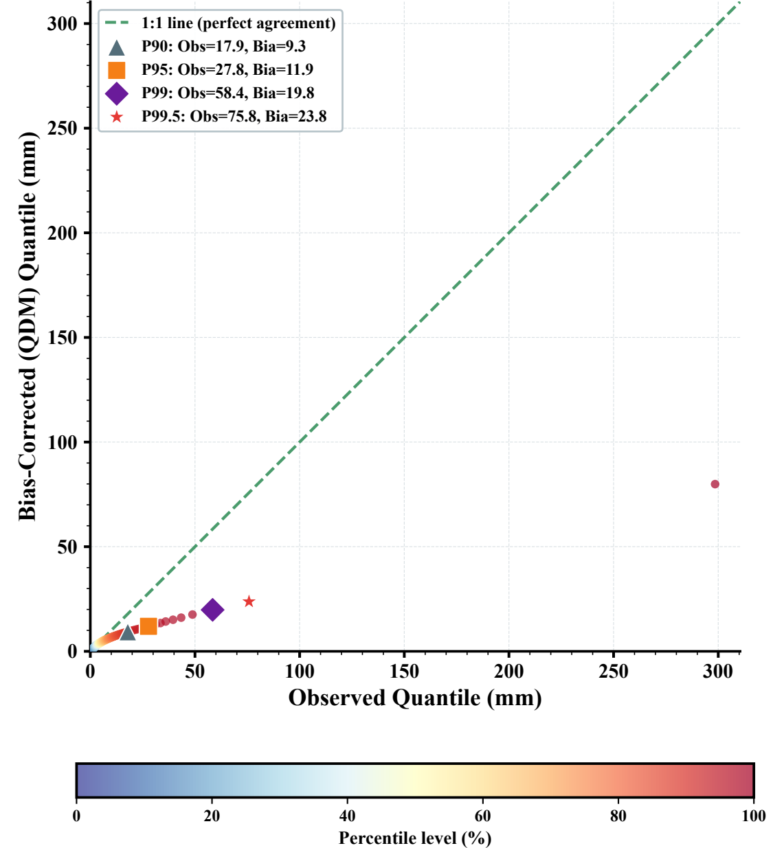
(b) Observed vs Bias-Corrected (QDM) QQ-RMSE = 17.02 mm
